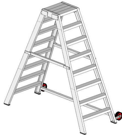
NBCP3056 A-Frame Ladder 2000mm
