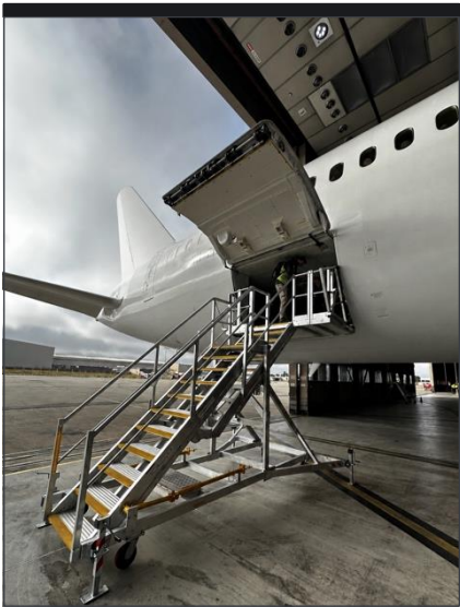
NBCP3129 A330/B787 Cargo Access
